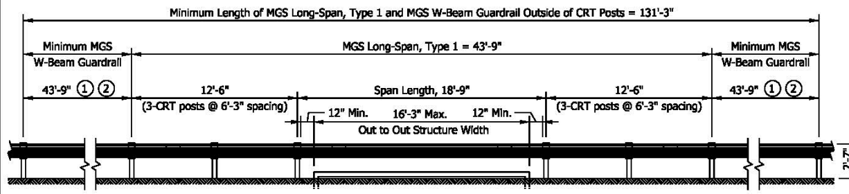
ELEVATION VIEW
